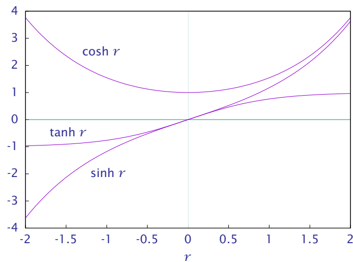
Figure 3: Hyperbolic trigonometric functions \sinh , \cosh and \tanh .
