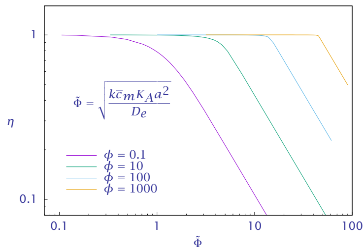
Figure 11: Effectiveness factor versus an inappropriate Thiele modulus in a slab; Hougen-Watson kinetics.
