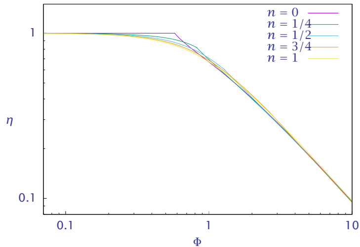
Figure 9: Effectiveness factor versus Thiele modulus in a spherical pellet; reaction orders less than unity.
