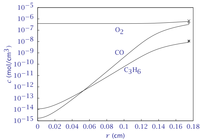
Figure 18: Concentration profiles of reactants (log scale); fluid concentration of O 2 (x), CO (+), C 3 H 6 (*).
