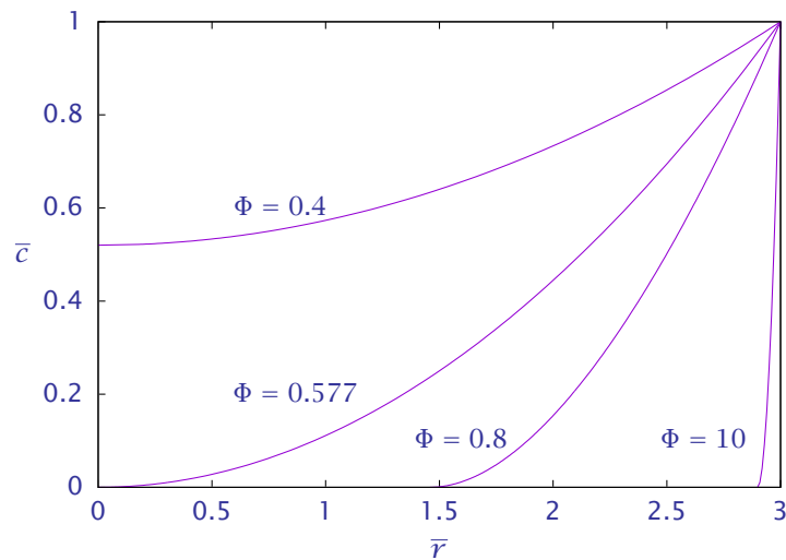
Figure 10: Dimensionless concentration versus radius for zero-order reaction ( n = 0 ) in a spherical pellet ( q = 2 ); for large \Phi the inner region of the pellet has zero A concentration.
