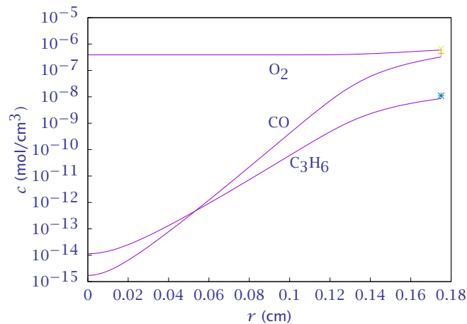
Figure 18: Concentration profiles of reactants (log scale); fluid concentration of O 2 (×), CO (+), C 3 H 6 (*).
