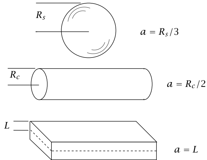
Figure 7: Characteristic length a for sphere, semi-infinite cylinder and semi-infinite slab.
