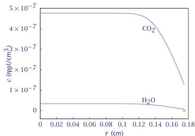
Figure 19: Concentration profiles of the products; fluid concentration of CO 2 (x), H 2 O (+).
