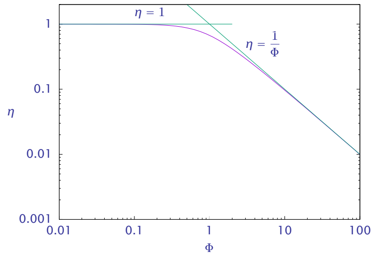
Figure 6: Effectiveness factor versus Thiele modulus for a first-order reaction in a sphere (log-log scale).
