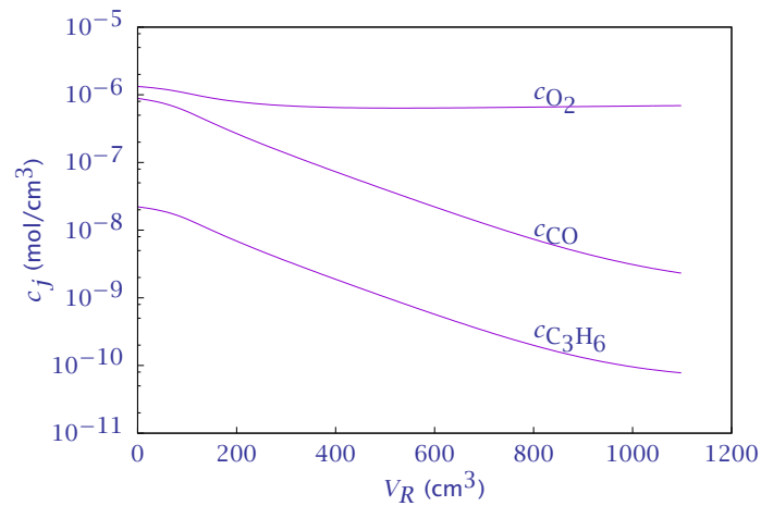
Figure 24: Fluid molar concentrations versus reactor volume.
