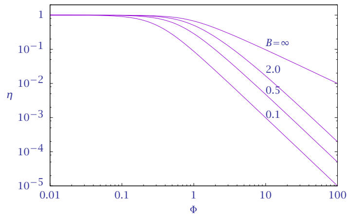
Figure 14: Effectiveness factor versus Thiele modulus for different values of the Biot number; first-order reaction in a spherical pellet.
