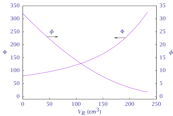
Figure 23: Dimensionless equilibrium constant and Thiele modulus versus reactor volume. Values indicate \eta = 1/\Phi is a good approximation for entire reactor.
