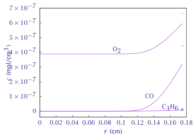
Figure 17: Concentration profiles of reactants; fluid concentration of O 2 (×), CO (+), C 3 H 6 (*).
