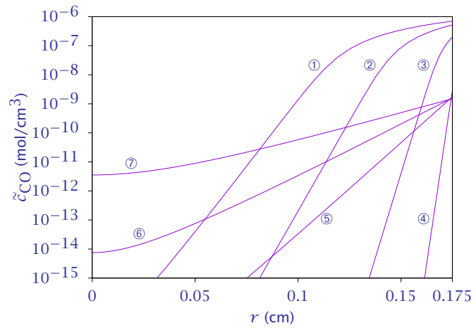
Figure 27: Pellet CO profiles at several reactor positions.
