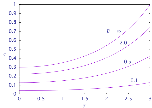
Figure 13: Dimensionless concentration versus radius for different values of the Biot number; first-order reaction in a spherical pellet with \Phi = 1 .
