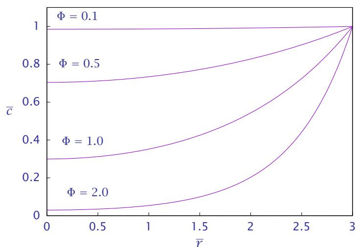
Figure 4: Dimensionless concentration versus dimensionless radial position for different values of the Thiele modulus.
