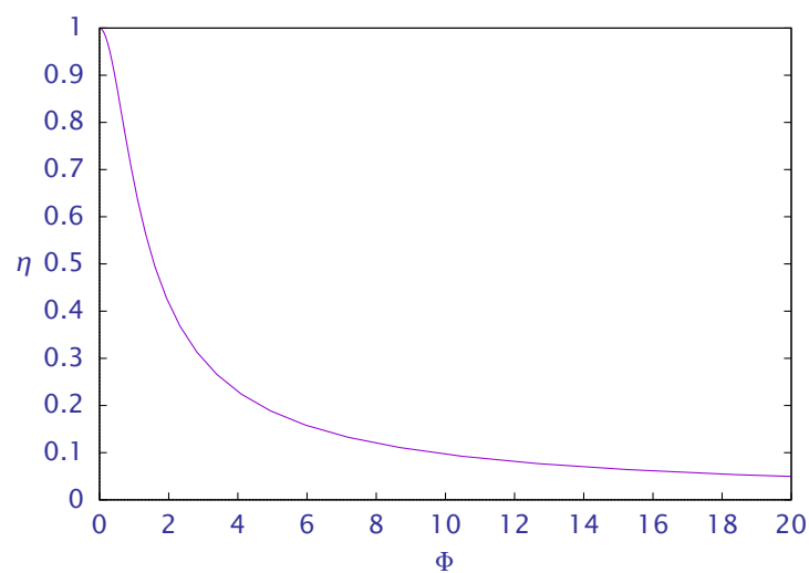
Figure 5: Effectiveness factor versus Thiele modulus for a first-order reaction in a sphere.
