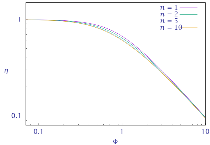
Figure 8: Effectiveness factor versus Thiele modulus in a spherical pellet; reaction orders greater than unity.
