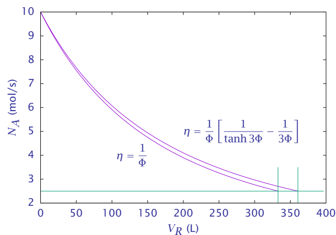
Figure 21: Molar flow of A versus reactor volume for second-order, isothermal reaction in a fixed-bed reactor.
