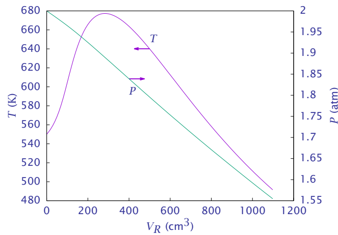
Figure 25: Fluid temperature and pressure versus reactor volume.
