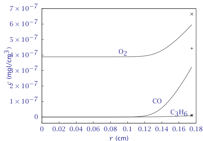
Figure 17: Concentration profiles of reactants; fluid concentration of O 2 (x), CO (+), C 3 H 6 (*).
