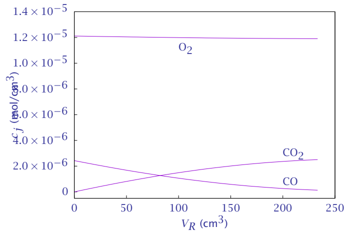
Figure 22: Molar concentrations versus reactor volume.
