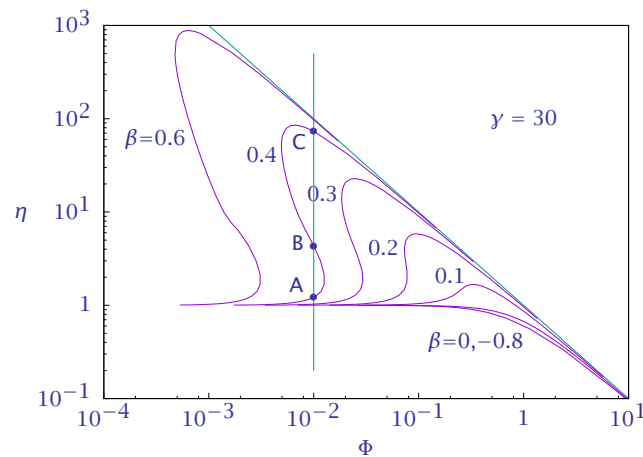
Figure 16: Effectiveness factor versus normalized Thiele modulus for a first-order reaction in a nonisothermal spherical pellet.
