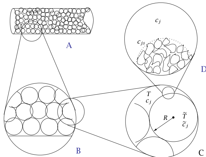
Figure 1: Expanded views of a fixed-bed reactor.
