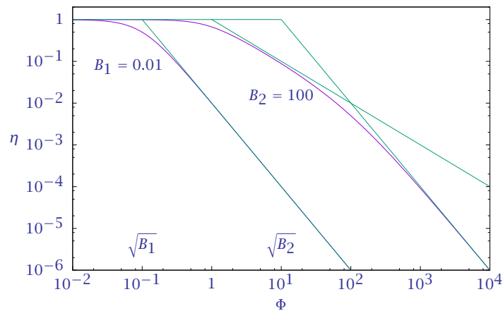
Figure 15: Asymptotic behavior of the effectiveness factor versus Thiele modulus; first-order reaction in a spherical pellet.
