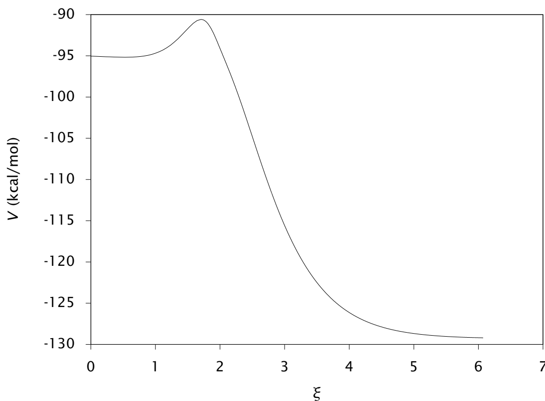
Figure 5.4: Reaction-coordinate diagram.
