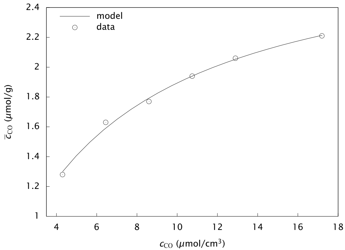
Figure 5.19: Langmuir isotherm for CO uptake on Ru.
