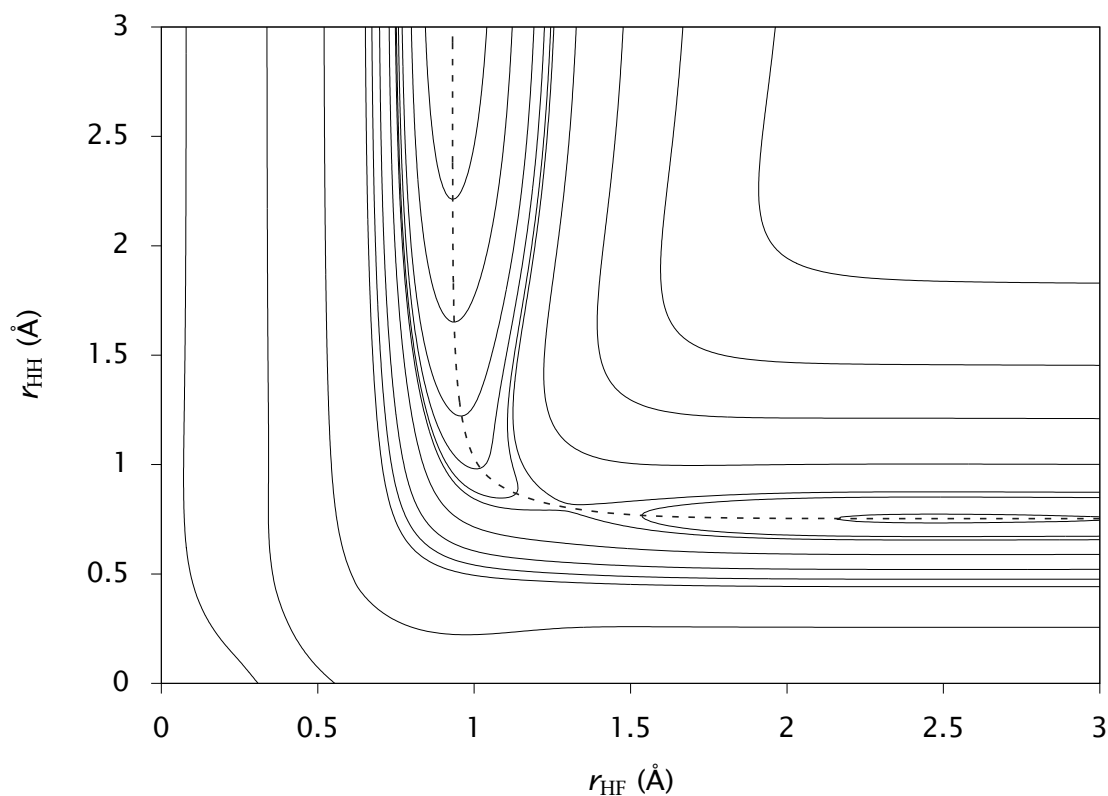
Figure 5.3: Contour representation of the potential-energy surface.
