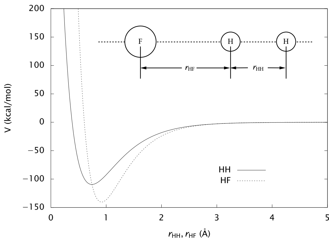
Figure 5.1: Morse potential for H 2 and HF.
